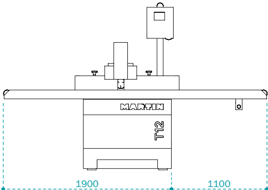
T12 | Side view
