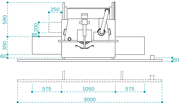
T12 | Plan view
