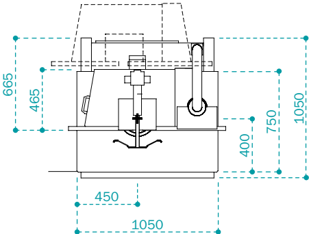
T12 | Plan view
