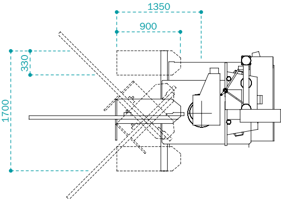
T12 with T1280 | Plan view
