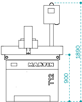
T12 | Side view
